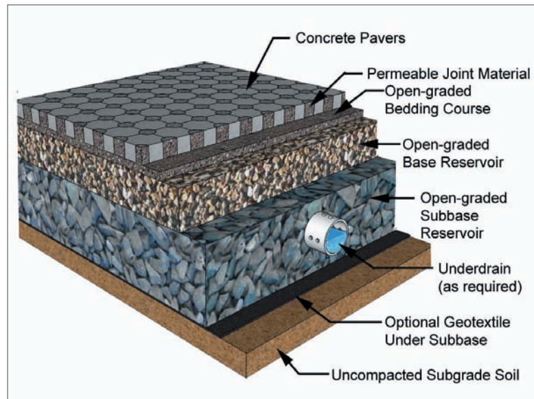
Typical PICP cross section
