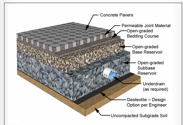
Typical PICP cross section
